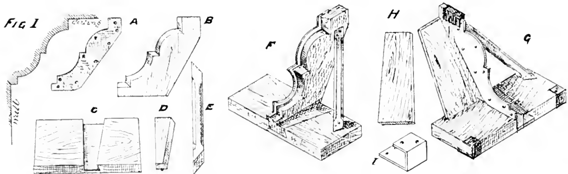
NO. 118.—TO MAKE A RUNNING MOULD.
